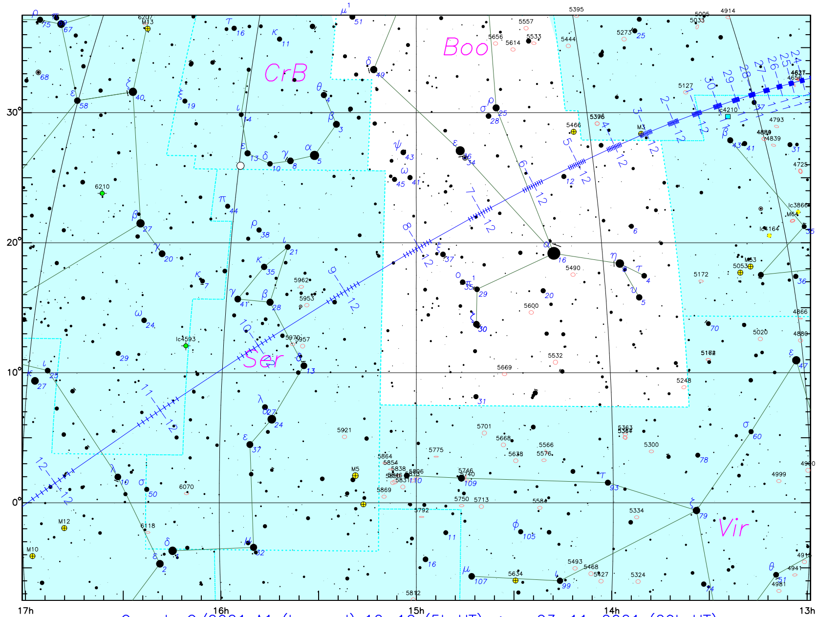
Comete C/2021 A1 (Leonard) 12-12 (5h UT) <-- 23-11-2021 (20h UT)
