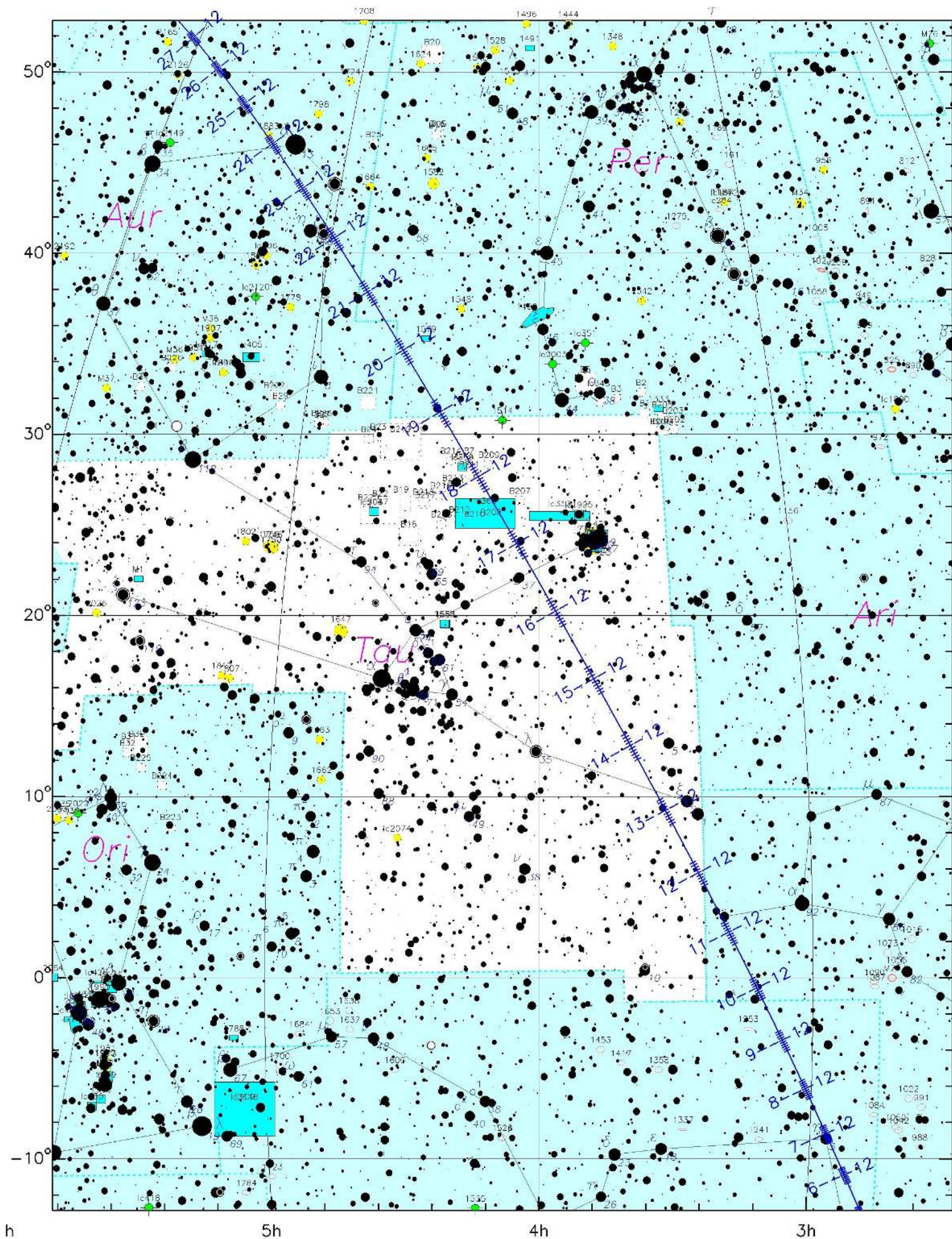
46P/Wirtanen (19h--4h UT)
