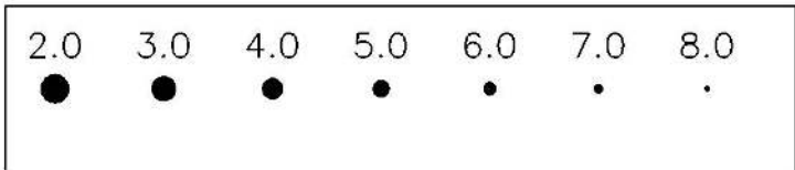
46P/Wirtanen (19h--4h UT)
