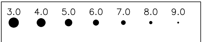
46P/Wirtanen (19h--4h UT)
