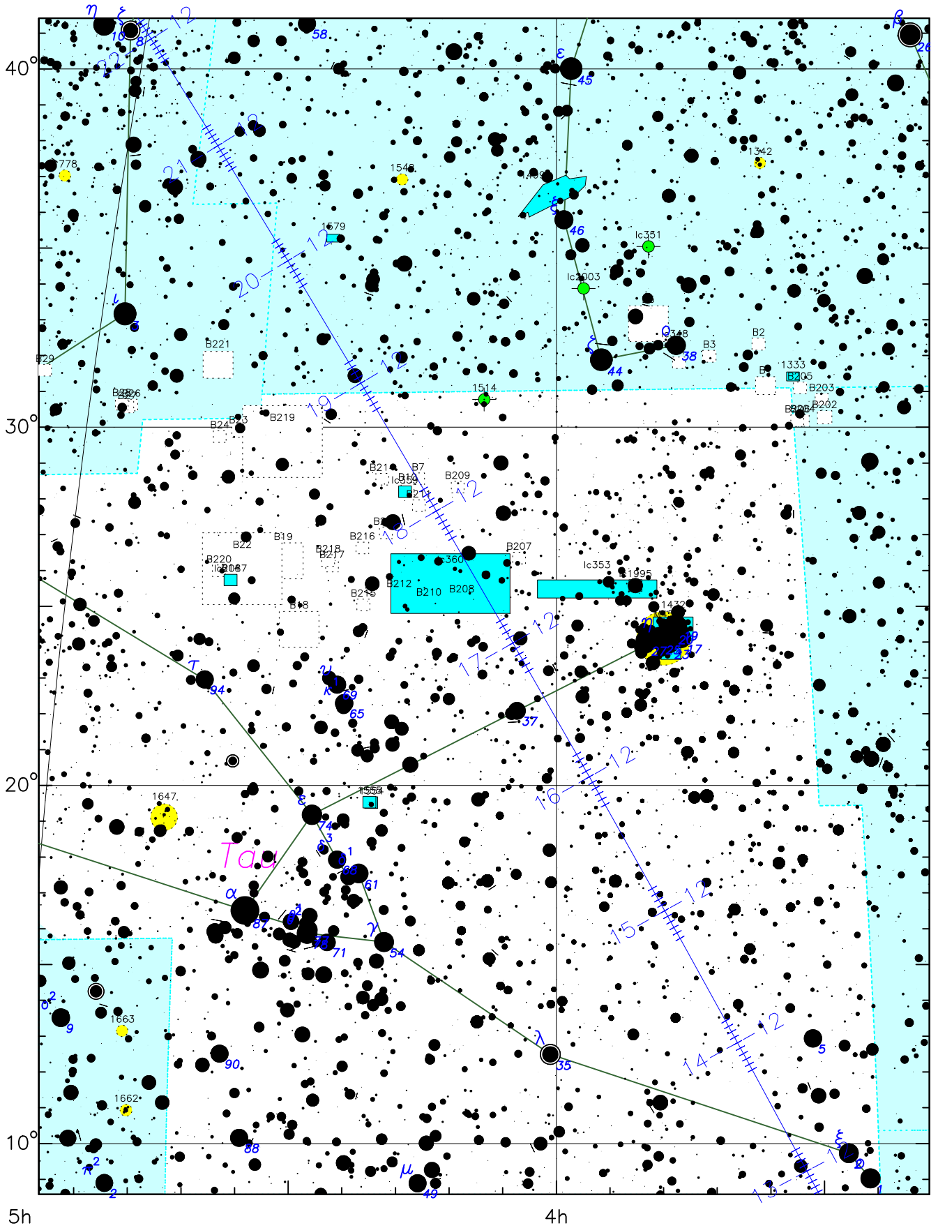
46P/Wirtanen (19h--4h UT)
